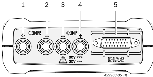
Abb. 2: Diagnosestrook/Meetstrook KTS 590
